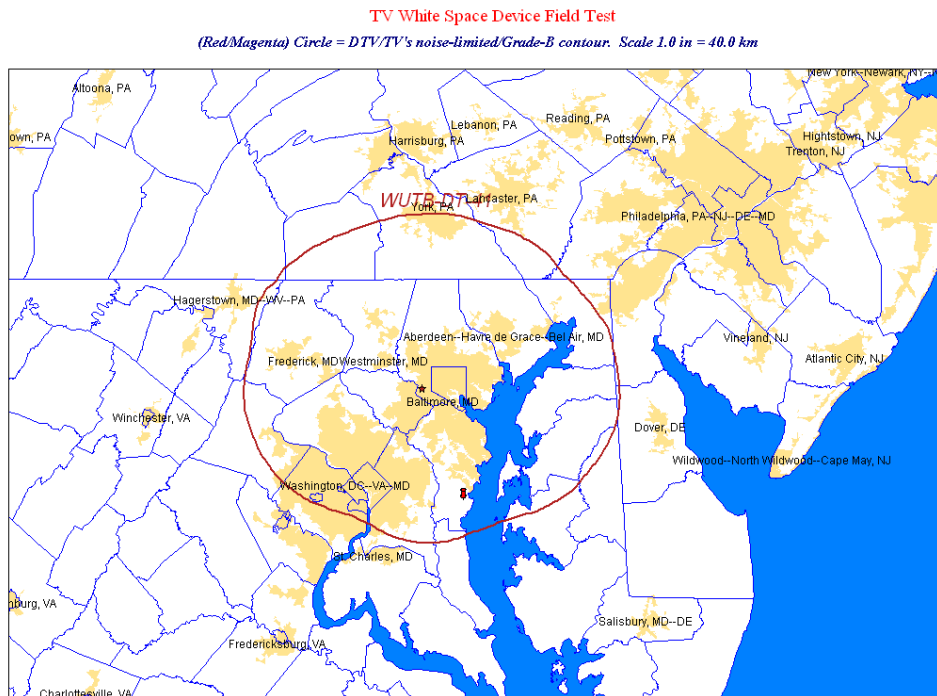
Figure D-184. Channel 41: WUTB-DT.
