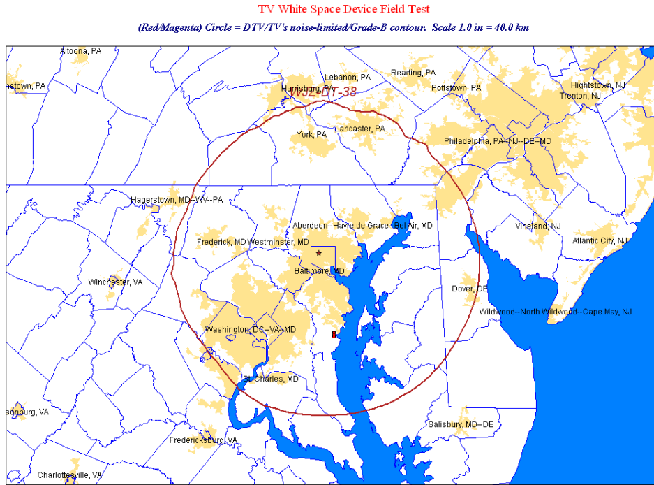
Figure D-181. Channel 38: WJZ-DT.
