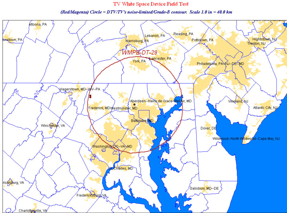
Figure D-205. Channel 29: WMPB-DT.
