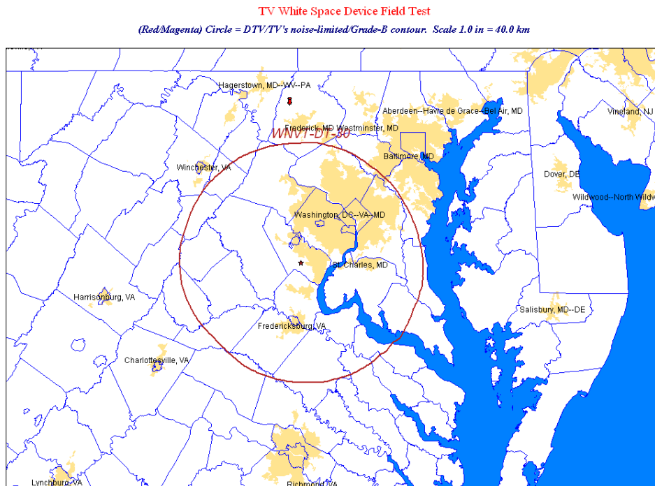
Figure D-206. Channel 30: WNVT-DT.
