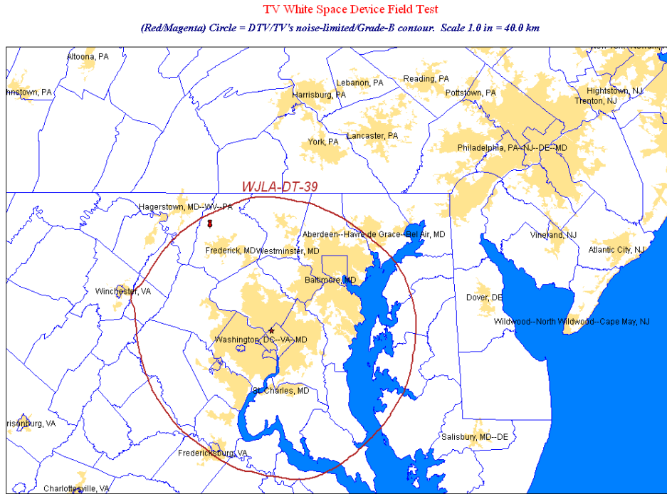
Figure D-215. Channel 39: WJLA-DT.
