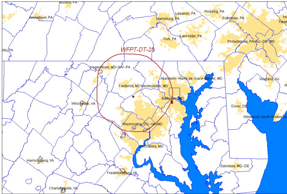
Figure D-42. Channel 28: WFPT-DT.
