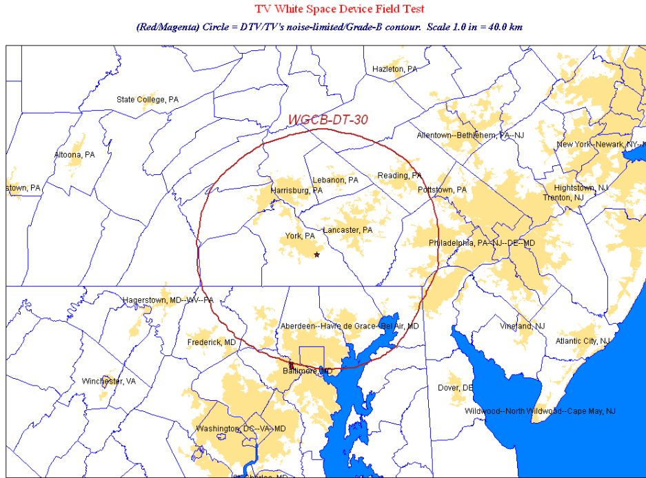
Figure D-77. Channel 30: WGCB-DT.
