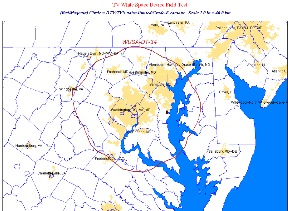
Figure D-178. Channel 34: WUSA-DT.
