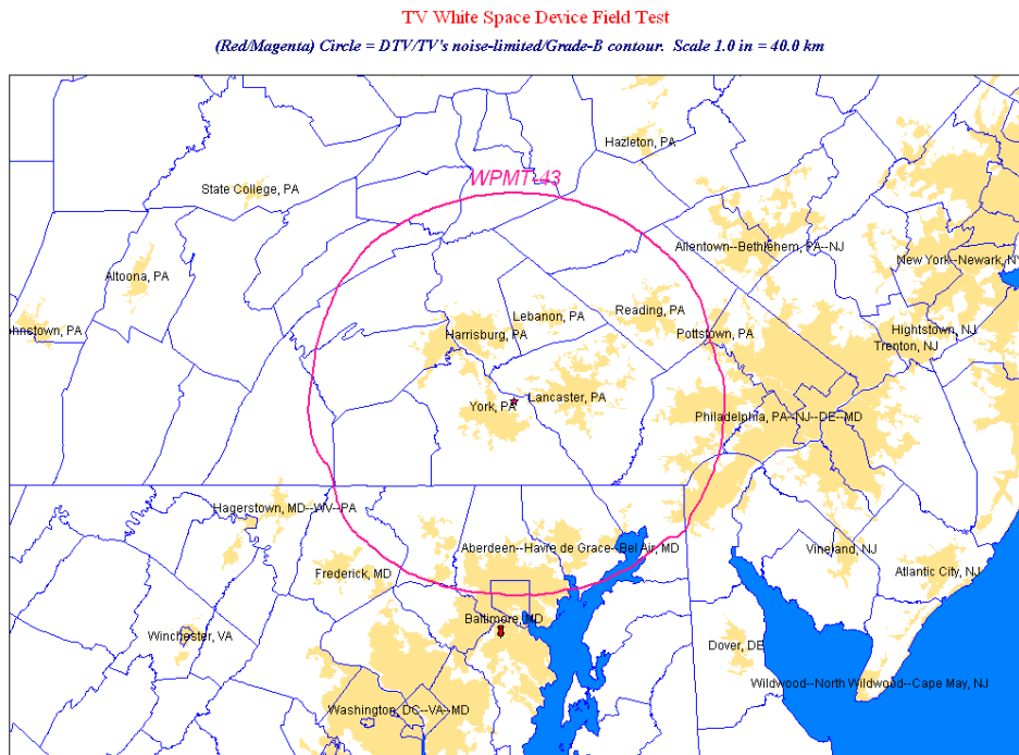
Figure D-57. Channel 43: WPMT-TV.
