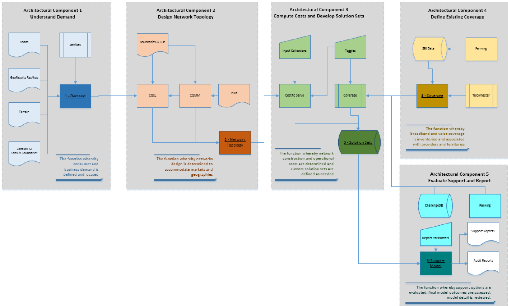
Figure 2--CACM Architecture
