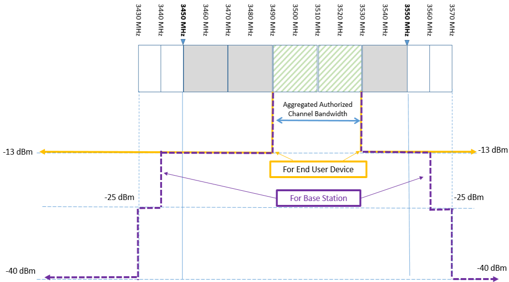
Figure 2: Emissions Mask
