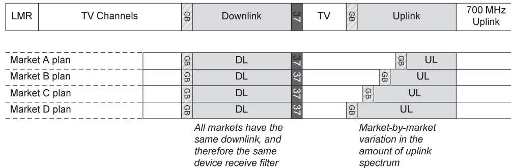
Figure 5. Fixed downlink with uplink varying by market
