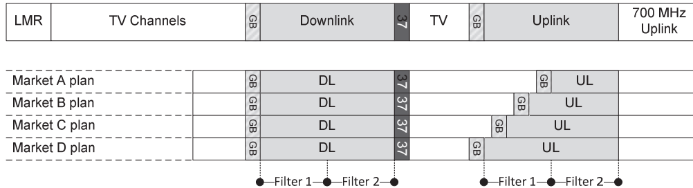
Figure 7. Example of family requiring two filters
