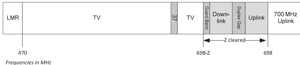
Figure 12. Alternative Approach, Down from 51
