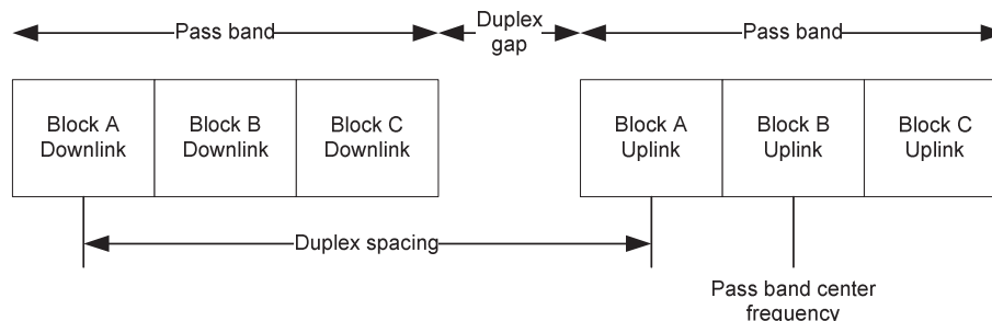
Figure 11. Illustration of duplexing terminology
