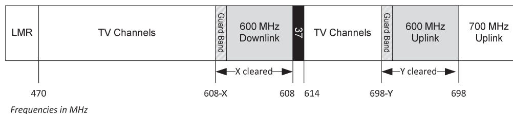
Figure 4. 600 MHz Band Plan
