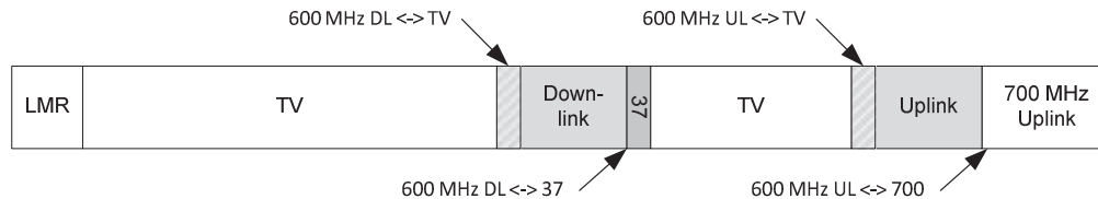
Figure 10. Guard band locations in the proposed band plan
