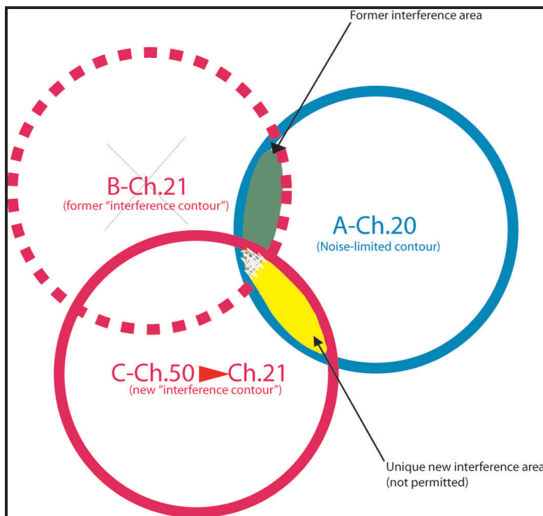
Figure 3: Illustration of “fixed” interference option
