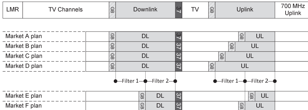
Figure 8. Two related plans based on aligning filters, an “extended family”
