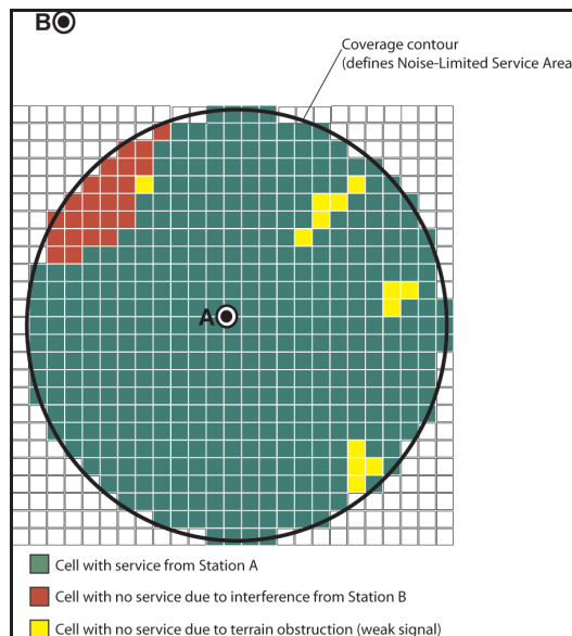
Figure 1. Illustration of OET Bulletin 69 coverage and interference
