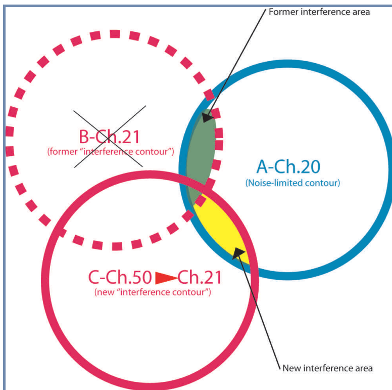
Figure 2: Illustration of “flexible” interference option
