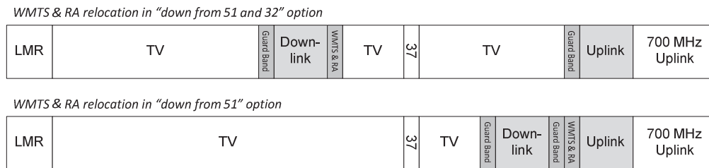
Figure 14. Alternatives, Relocation of Channel 37
