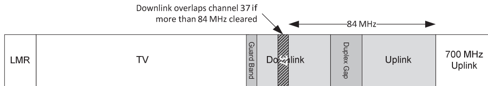
Figure 13. Impact of Fixed 37 on Down from 51 Alternative Approach
