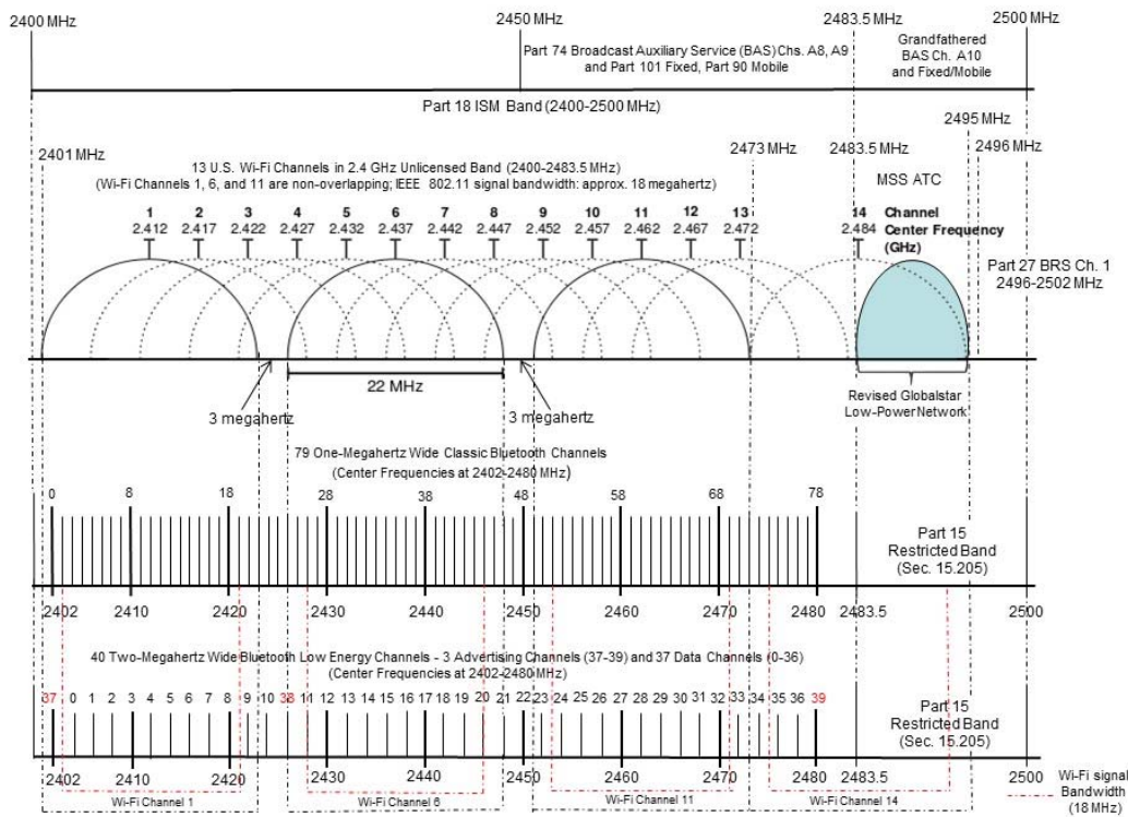
Overview of U.S. Channels in 2.4 GHz Unlicensed Band (2400-2483.5 MHz)
