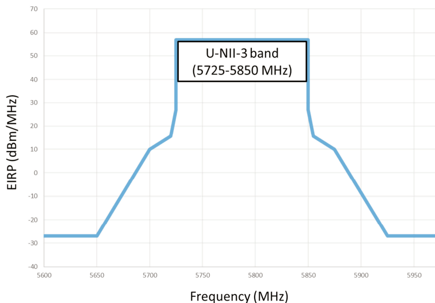
Figure 1. Proposed emission mask
